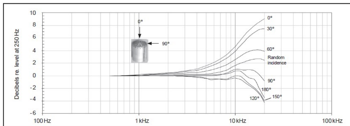
Free-field corrections for different angles of incidence
