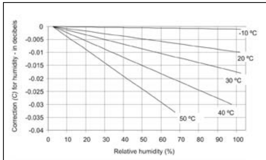
Fig. A.2 Corrections for temperature humidity
