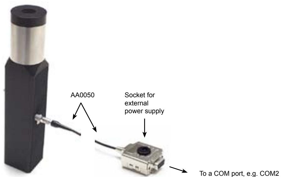
Fig. 4.1 Pistonphone connection to computer
